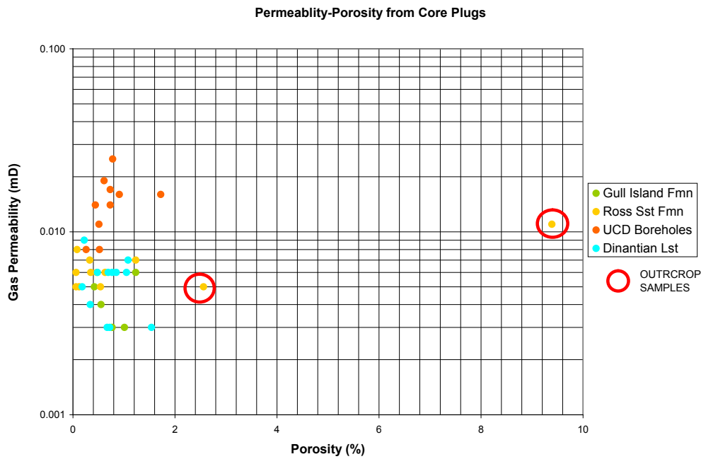
Figure 7.1. Permeability versus porosity plot for project and UCD data sets (outcrop samples highlighted). Fmn (formation), Sst (sandstone), Lst (limestone).
