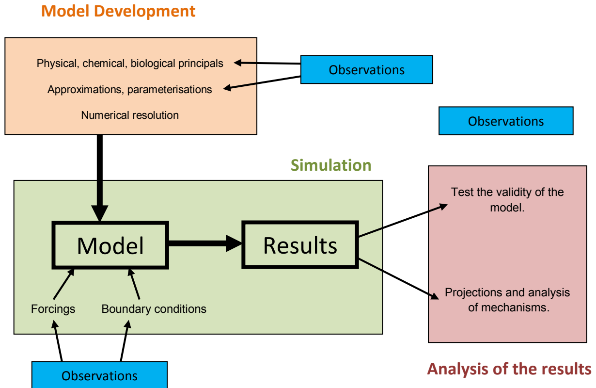
Figure 2.4. Schematic representation of the development and use of a climate model.
