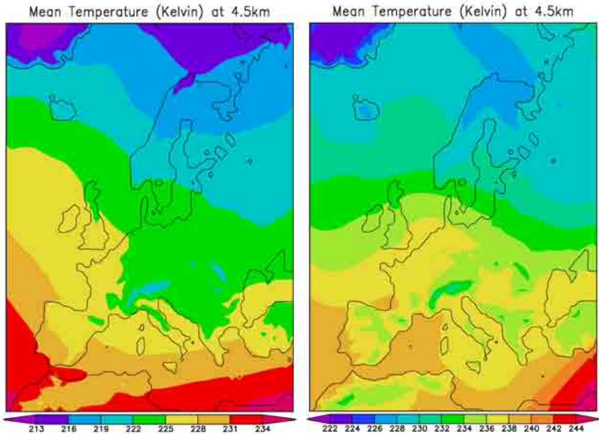
Figure 5.2. Modelled temperatures for January (left) and June 2003 (right) at 4.5 km.
