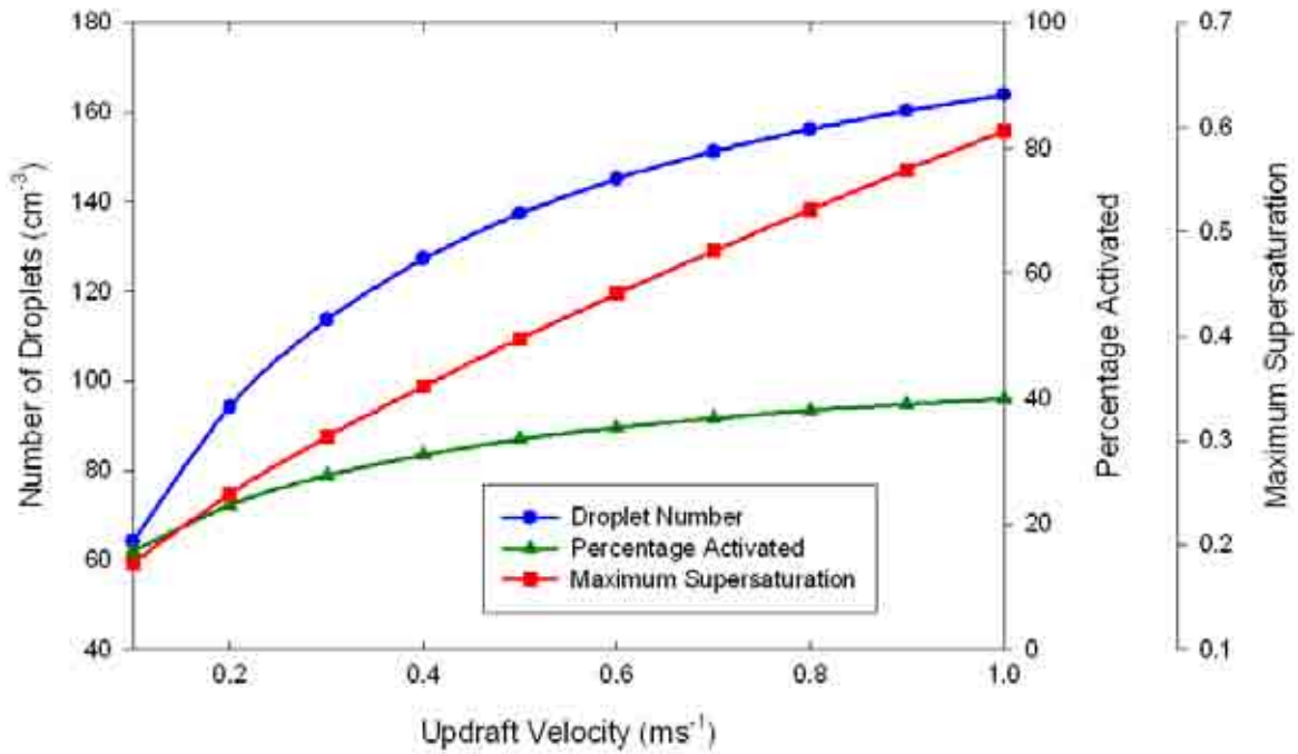
Figure 4.4. Sample output from the cloud droplet activation parameterisation. The blue line gives the cloud droplet number, the green line gives the percentage of cloud condensation nuclei activated and the red line gives the maximum supersaturation for different values of updraft velocity.
