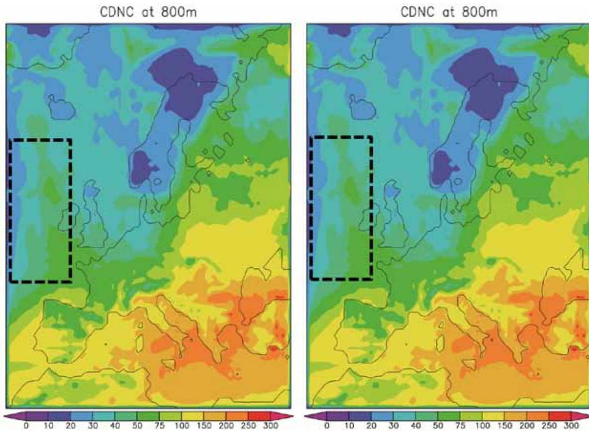
Figure 5.4. The average cloud droplet number concentration in cm -3 over Europe and the north Atlantic for the months of January (left) and June (right) 2003. Area M1 is the area within the dashed black line.
