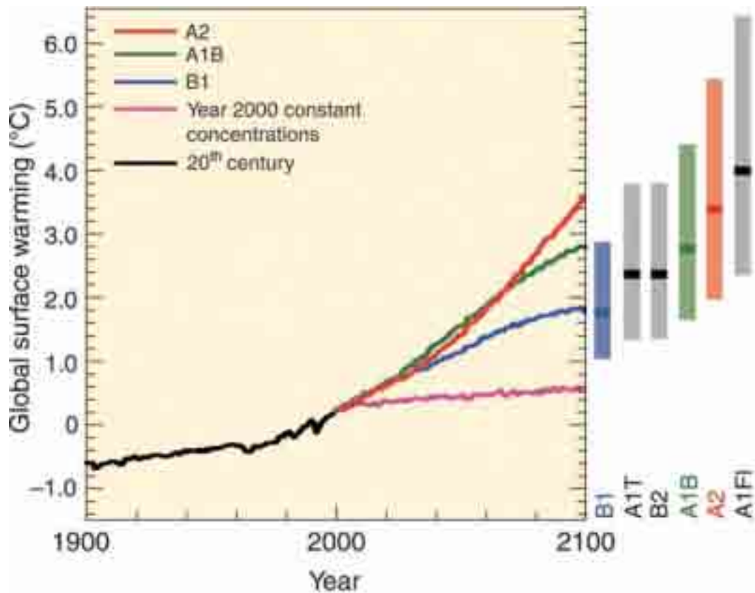
Figure 2.1. Solid lines are multi-model global averages of surface warming (relative to 1980–1999) for the emission scenarios, shown as continuations of the 20th century simulations. The B1 scenario describes a world more integrated, and more ecologically friendly than present day. A1T represents a future reliant on non-fossil fuel energy sources. B2 represents a world of increased concern for environmental and social sustainability. A1B represents a future where there is a balance across all fuel sources. The A2 scenario represents a more divided world and A1FI represents a fossil intensive future. The pink line is for the experiment where concentrations were held constant at year 2000 values. For a full explanation of the scenarios see Nakićenović and Swart (2000). (From IPCC, 2007.)
