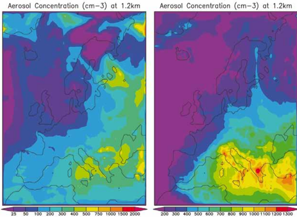
Figure 5.3. Modelled aerosol number concentrations for January (left) and June (right) 2003 at 1.2 km.
