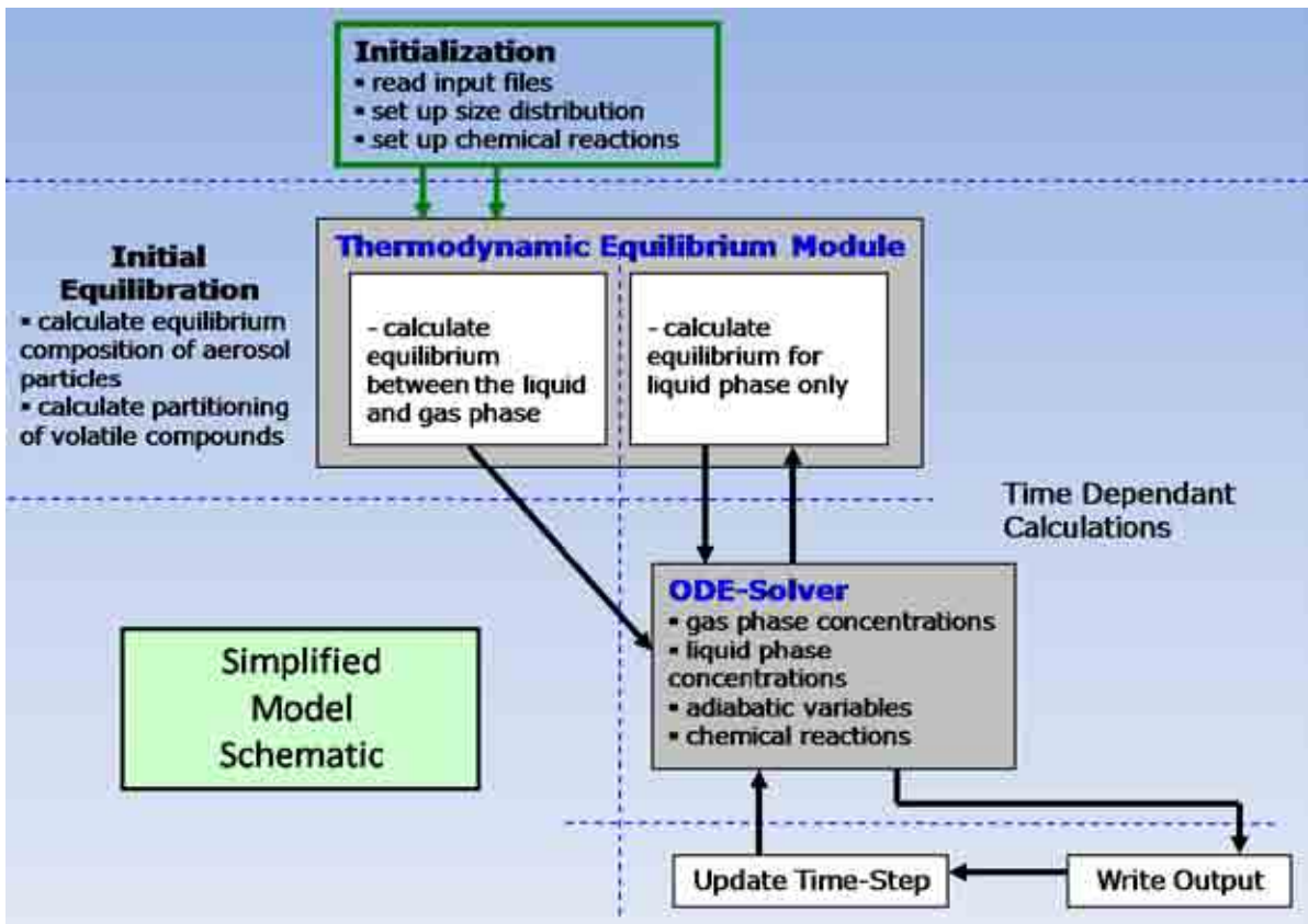
Figure 4.1. A simplified schematic of the aerosol–cloud chemistry process model.
