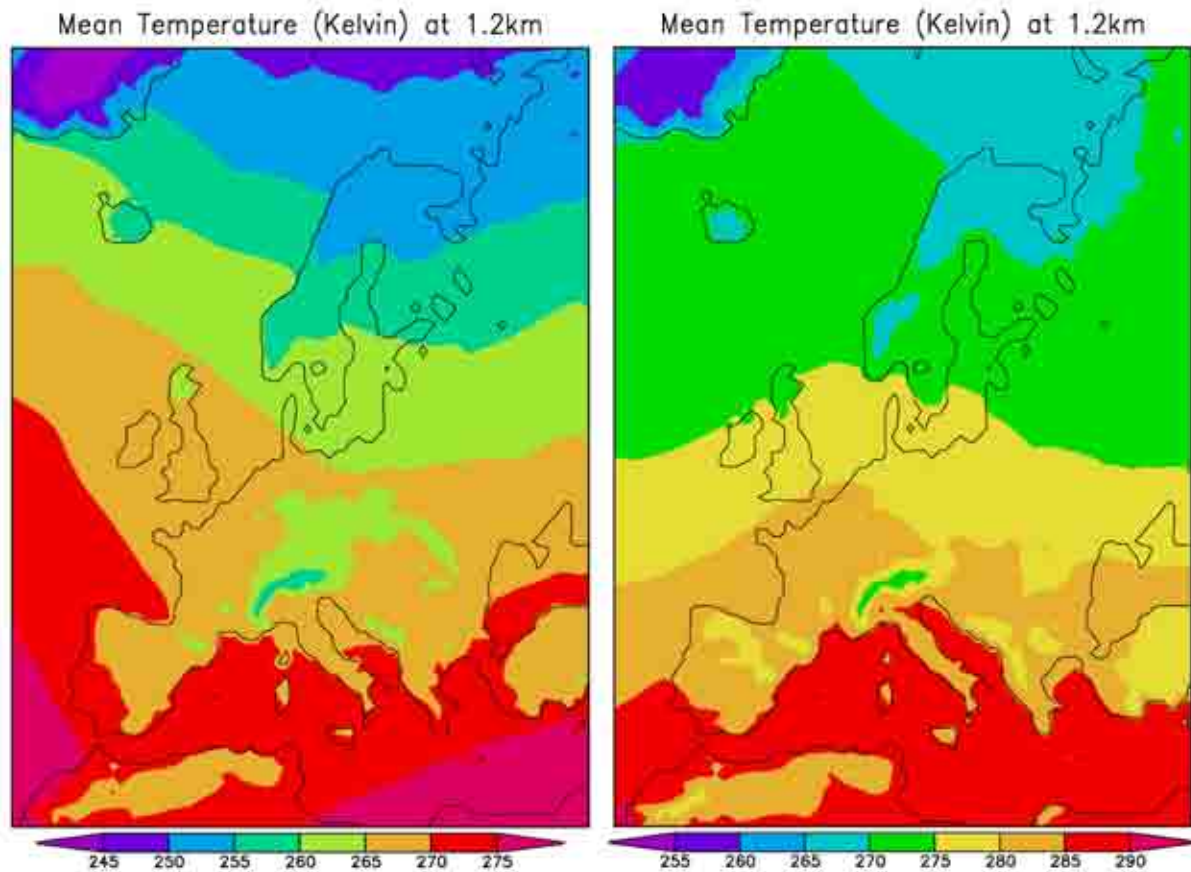
Figure 5.1. Modelled temperatures for January (left) and June (right) 2003 at 1.2 km.
