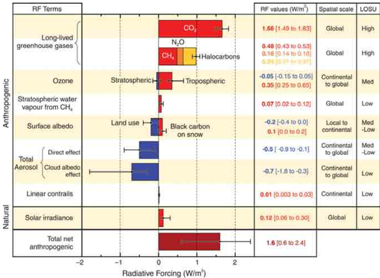
Figure 2.2. Global average radiative forcing (RF) estimates and ranges in 2005 for anthropogenic carbon dioxide (CO 2 ), methane (CH 4 ), nitrous oxide (N 2 O) and other important agents and mechanisms, together with the typical geographical extent (spatial scale) of the forcing and the assessed level of scientific understanding (LOSU). The net anthropogenic radiative forcing and its range are also shown. (Taken from Solomon et al., 2007.)
