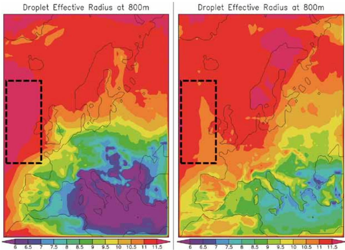
Figure 5.5. The average droplet effective radius in \mu\text{m} over Europe and the north Atlantic for the months of January (left) and June (right) 2003. Area M1 is the area within the dashed black line.
