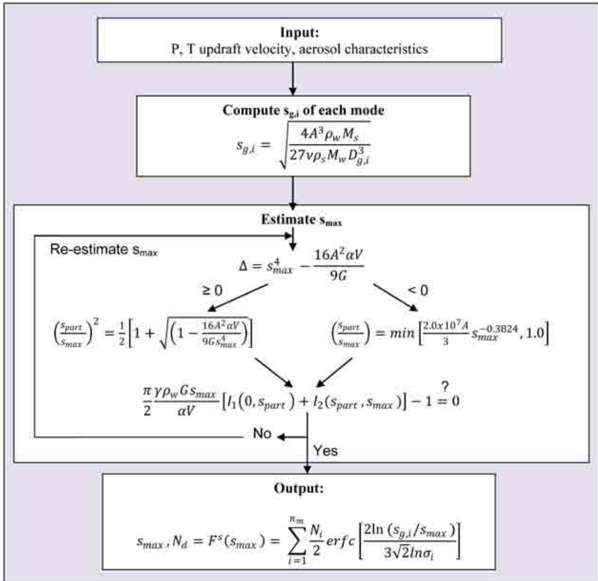
Figure 4.3. An overview of the algorithm used in the parameterisation (adapted from Fountoukis et al., 2005).
