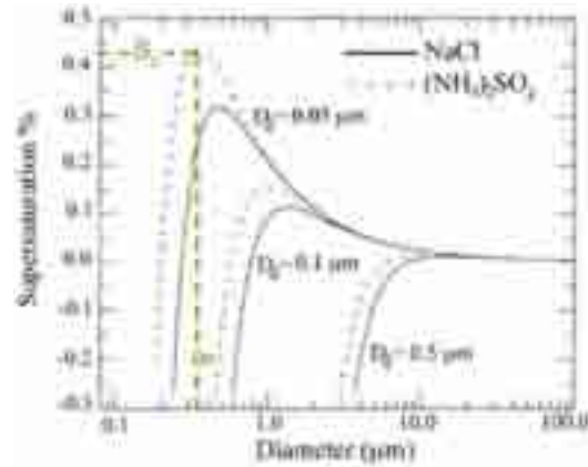
Figure 2.3. Ammonium sulphate and sodium chloride Köhler curves.
