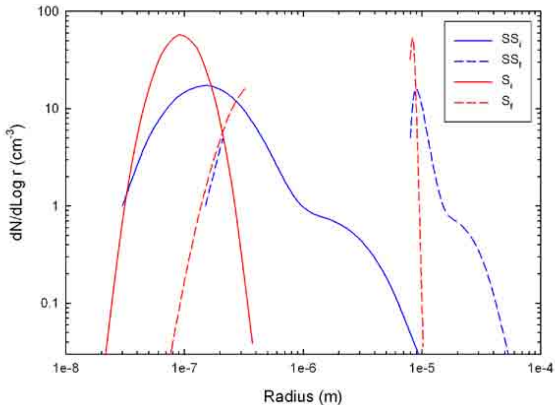
Figure 4.2. Sulphate (S) and sea-salt (SS) aerosol distributions before (left) and after (right) a cloud cycle. Here the subscripts i and f stand for initial and final, respectively. dN/d\log r is the number of particles per \text{cm}^3 of air in the size range \log r to (\log r + d\log r) where r refers to particle radius.
