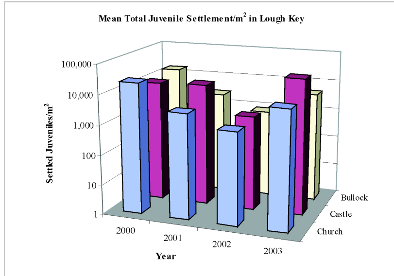
Figure 3.3. Total mean juvenile settlement for July and August in Lough Key, 2000–2003.
