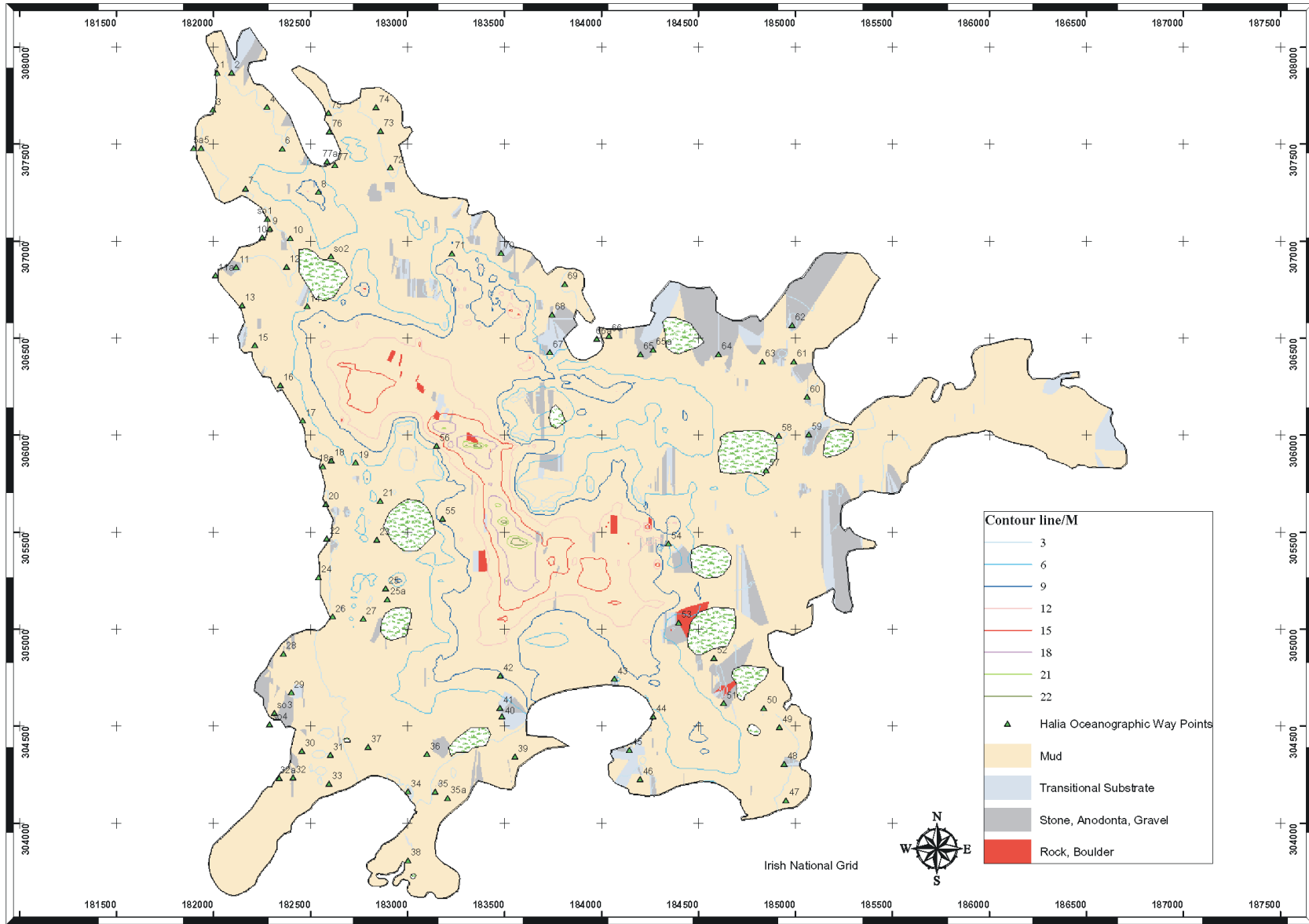
Figure 3.1. Map of Lough Key showing the four main substrates and depth at 3-m contour levels.
