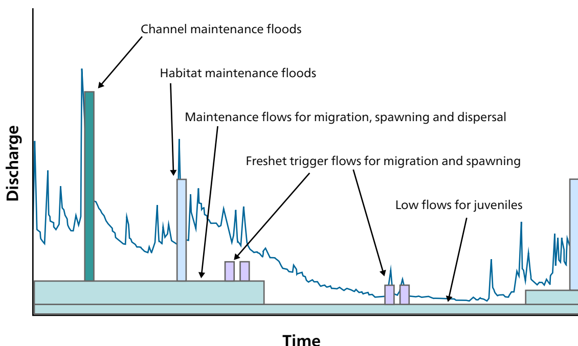
Figure 5 Conceptual “building block” flow components required to deliver the environmental supporting conditions in rivers (SNIFFER, 2007)
