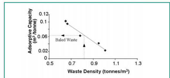
FIGURE 7.3: RELATIONSHIP BETWEEN WASTE DENSITY AND THE ABSORPTIVE CAPACITY OF WASTE
