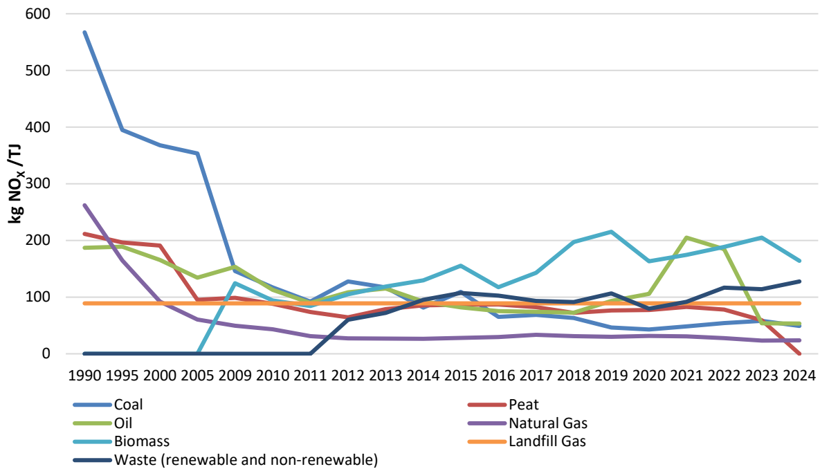
Figure 3.1 Nitrogen Oxide (NO x ) Implied Emission Factors (IEFs) for Category 1A1a
