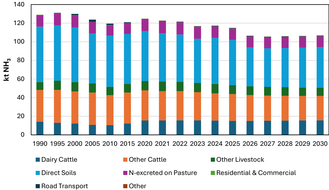
Figure 8.7 NH 3 Emission Projections for the With Additional Measures Scenario by Source Sector
