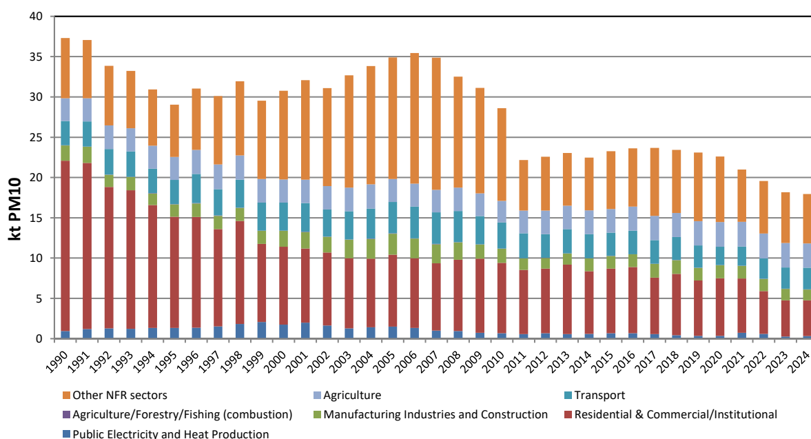
Figure 2.6 Emission Trend for Particulate Matter <10 µm in Diameter 1990–2024
