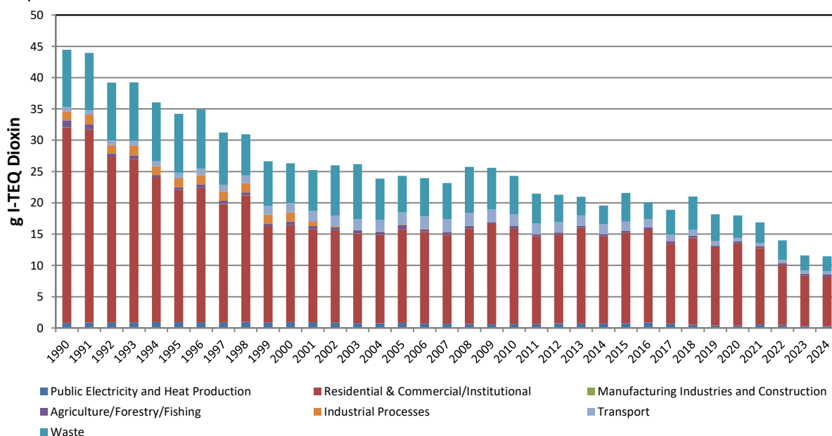
Figure 2.19 Emission Trend for Dioxins and Furans 1990–2024
