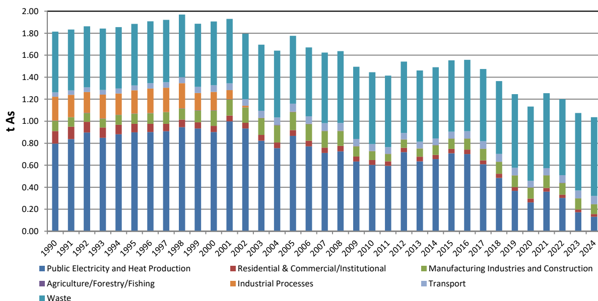
Figure 2.13 Emission Trend for Arsenic 1990–2024
