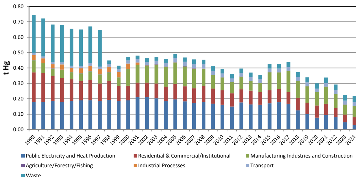
Figure 2.12 Emission Trend for Mercury 1990–2024
