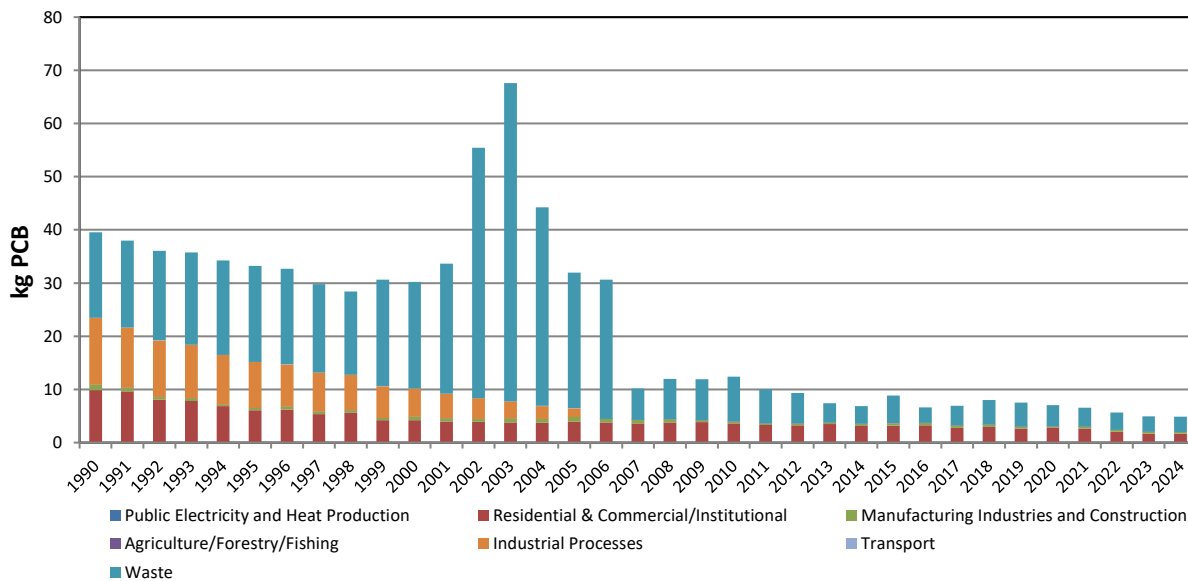
Figure 2.21 Emission Trend for Polychlorinated Biphenyls 1990–2024
