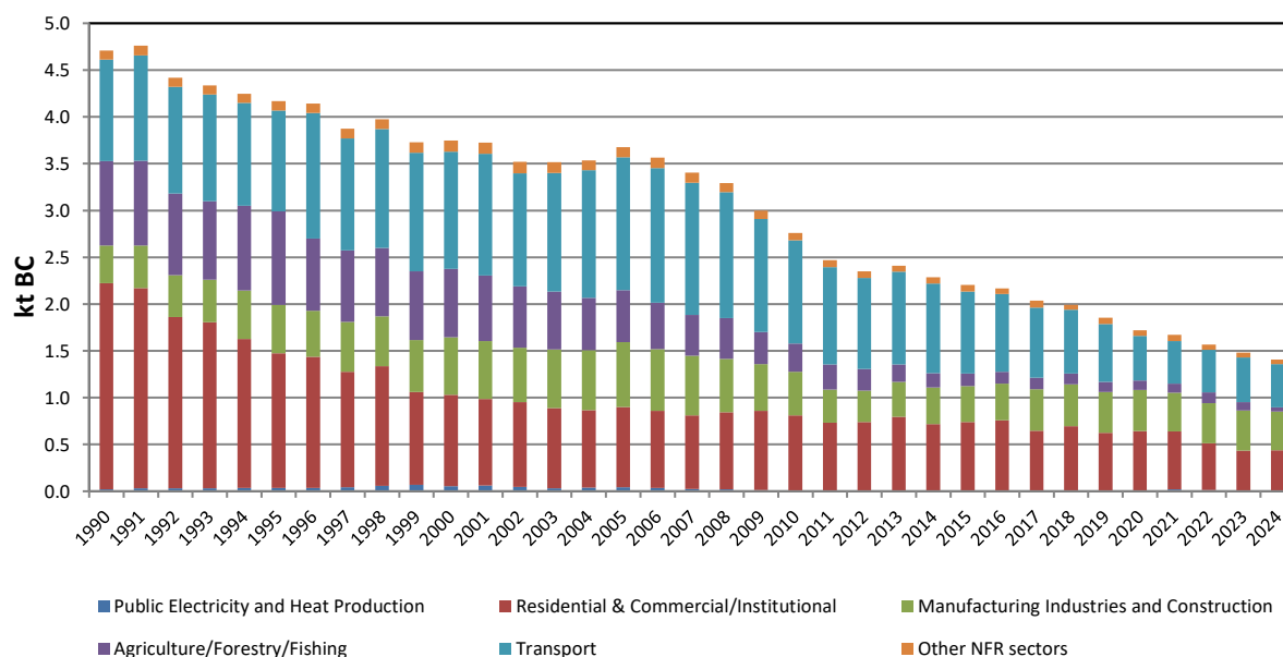
Figure 2.9 Emission Trend for Black Carbon 1990–2024
