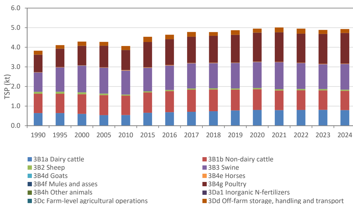
Figure 5.6. Emissions Trend for TSP from Agriculture 1990–2024
