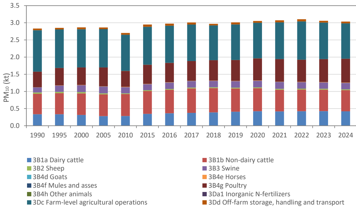
Figure 5.5. Emissions Trend for PM 10 from Agriculture 1990–2024
