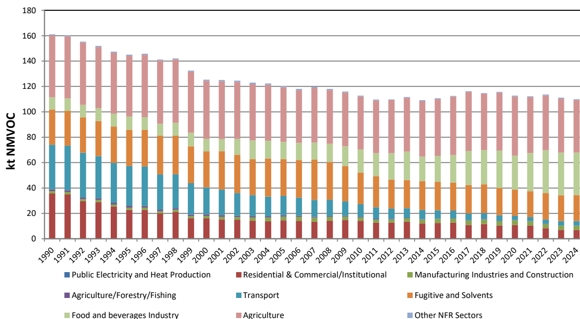
Figure 2.4 Emission Trend for Non-Methane Volatile Organic Compounds 1990–2024
