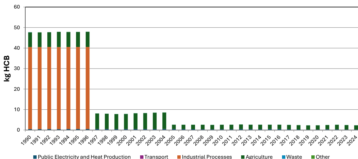
Figure 2.20 Emission Trend for Hexachlorobenzene 1990–2024
