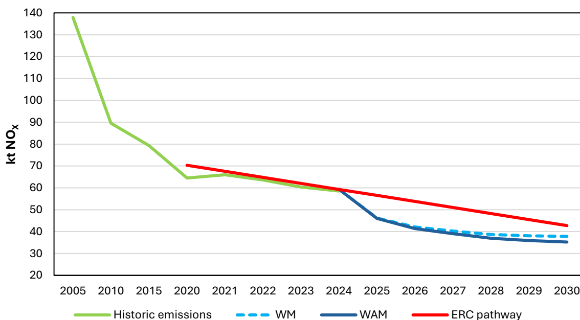
Figure 8.4 NO x Emission Projections for the With Existing Measures and With Additional Measures Scenarios under the Gothenburg Protocol (without 3D)
