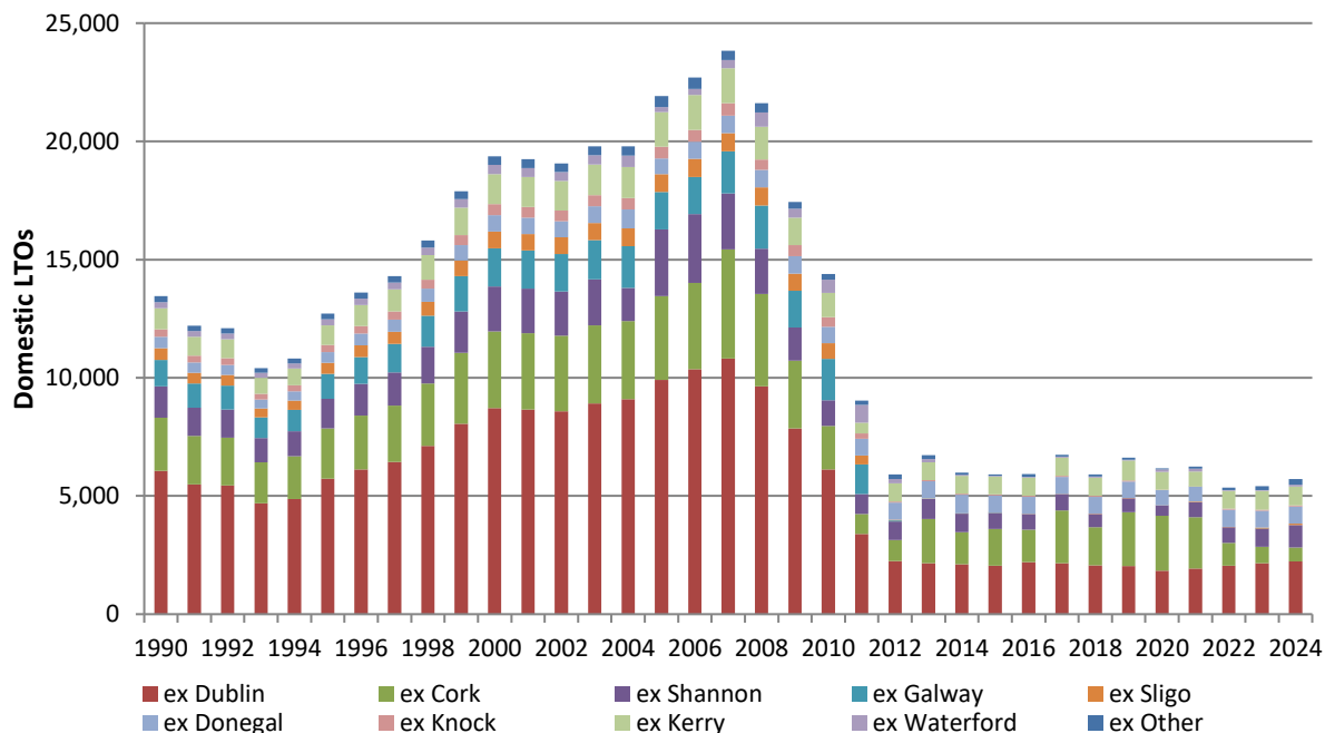
Figure 3.3 Number of Domestic LTOs from Irish airports 1990-2024
