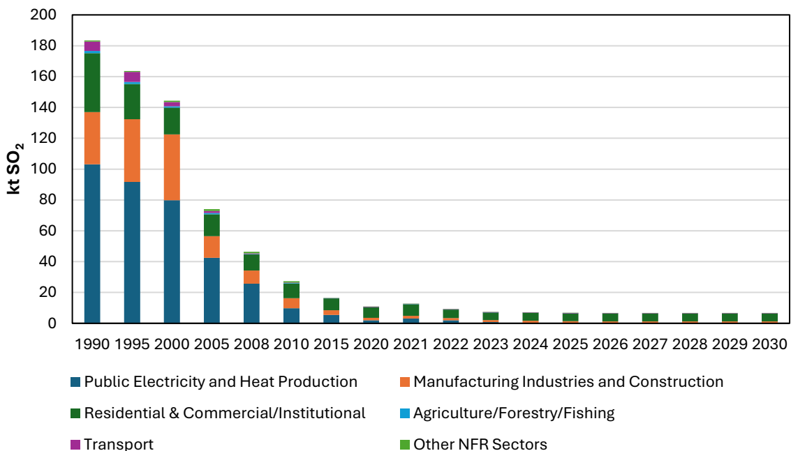
Figure 8.2 SO 2 Emission Projections for the With Additional Measures Scenario by Source Sector
