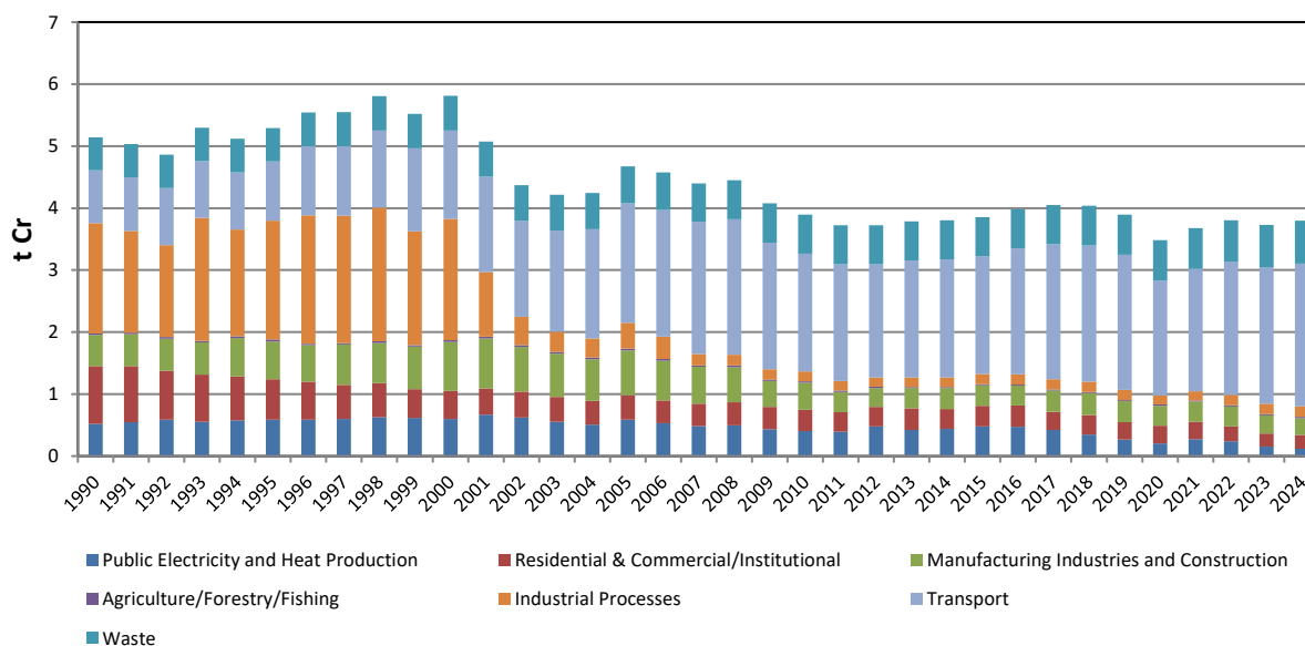
Figure 2.14 Emission Trend for Chromium 1990–2024
