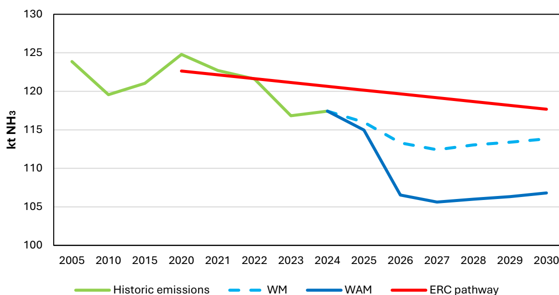
Figure 8.6 NH 3 Emission Projections for the With Existing Measures and With Additional Measures Scenarios
