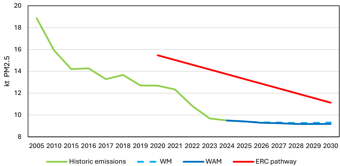
Figure 8.12 PM 2.5 Emission Projections for the With Existing Measures and With Additional Measures Scenarios
