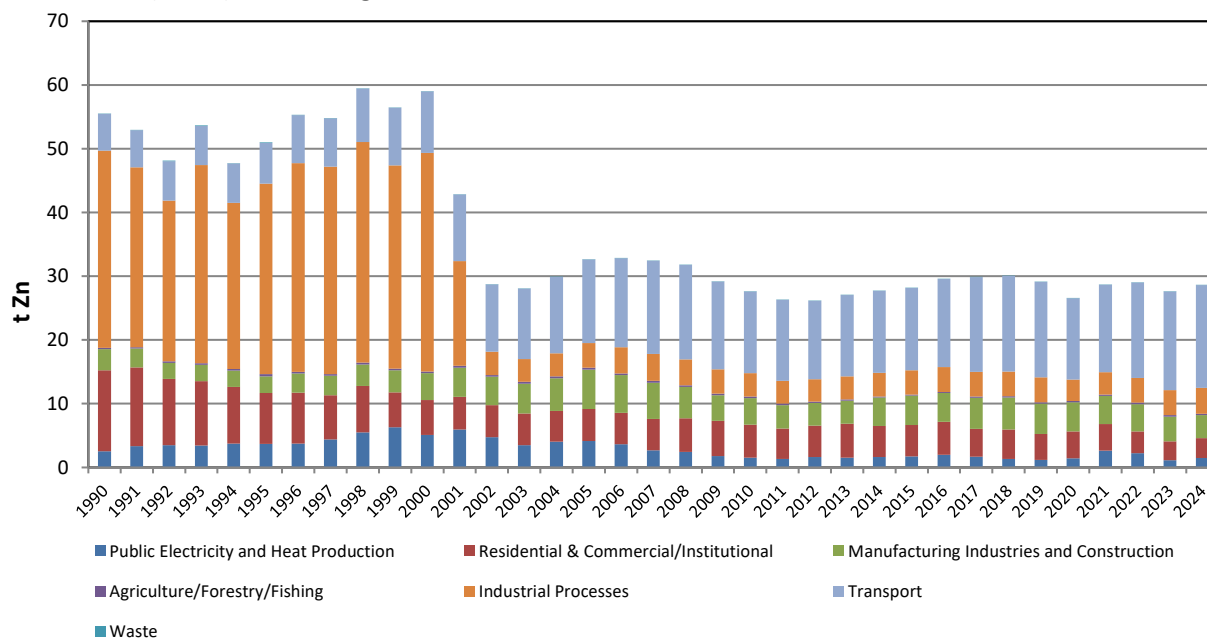
Figure 2.18 Emission Trend for Zinc 1990–2024
