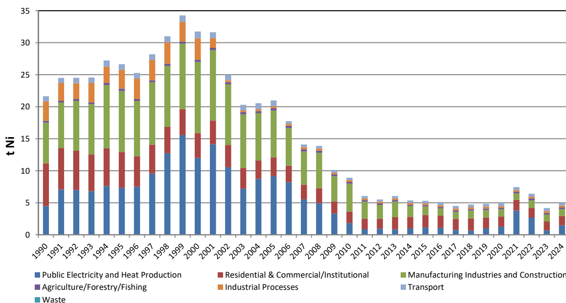
Figure 2.16 Emission Trend for Nickel 1990–2024
