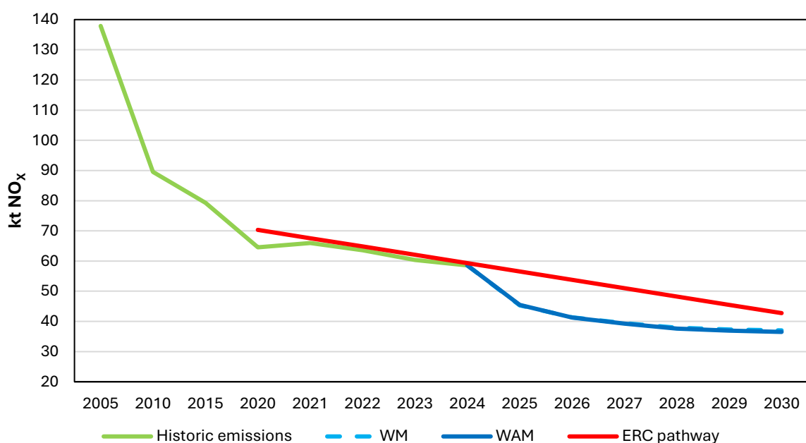
Figure 8.3 NO x Emission Projections for the With Existing Measures and With Additional Measures Scenarios under NECD (without 3B and 3D)
