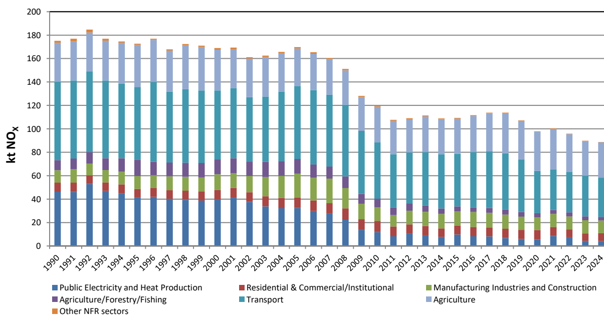
Figure 2.2 Emission Trend for Nitrogen Oxides 1990–2024
