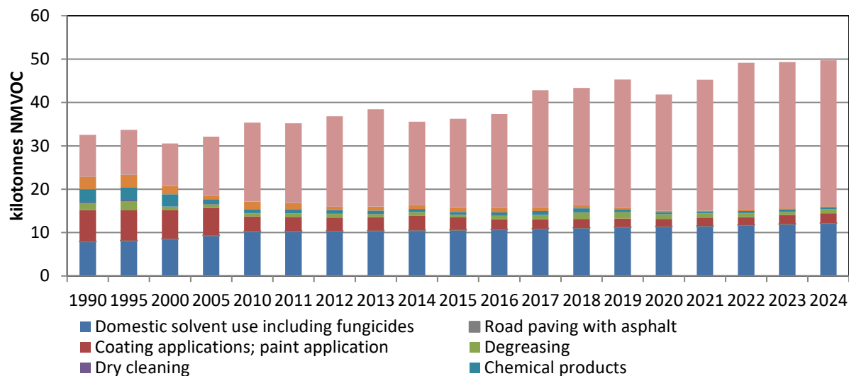
Figure 4.1 NMVOC Emission Trend for 2D-2H Other Solvent and Product 1990–2024
