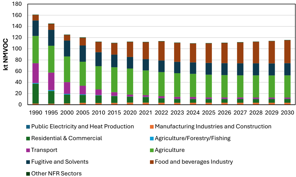
Figure 8.10 NMVOC Emission Projections for the With Additional Measures Scenario by Source Sector
