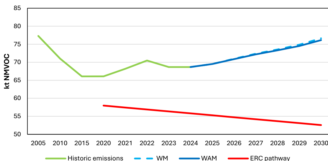
Figure 8.8 NMVOC Emission Projections for the With Existing Measures and With Additional Measures Scenarios 11 under NECD (without 3B and 3D)
