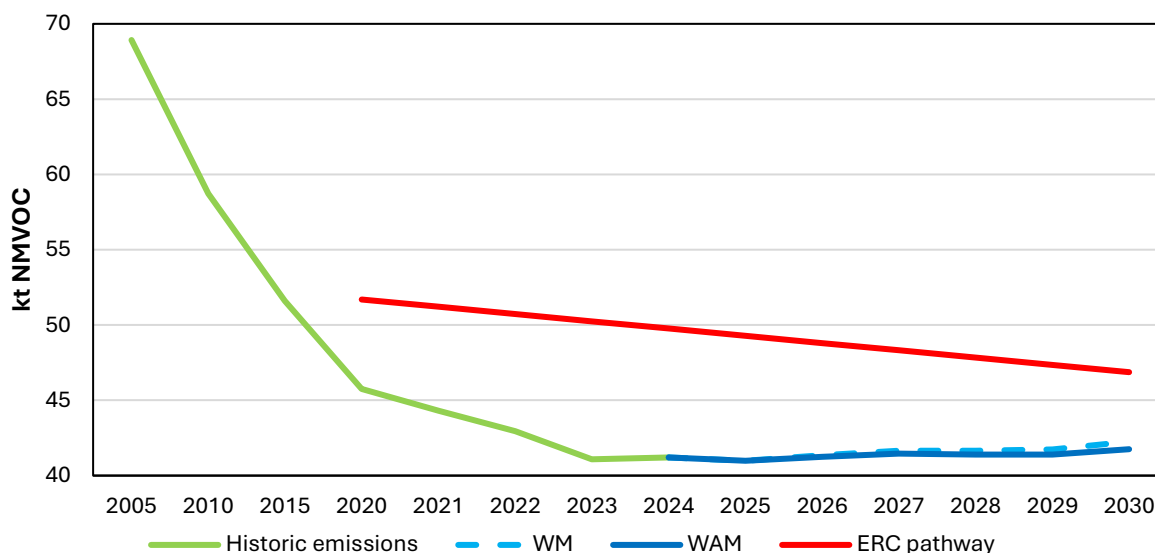
Figure 8.9 NMVOC Emission Projections for the With Existing Measures and With Additional Measures Scenarios where an adjustment is applied for category 2H2 Spirit production 12 under NECD
