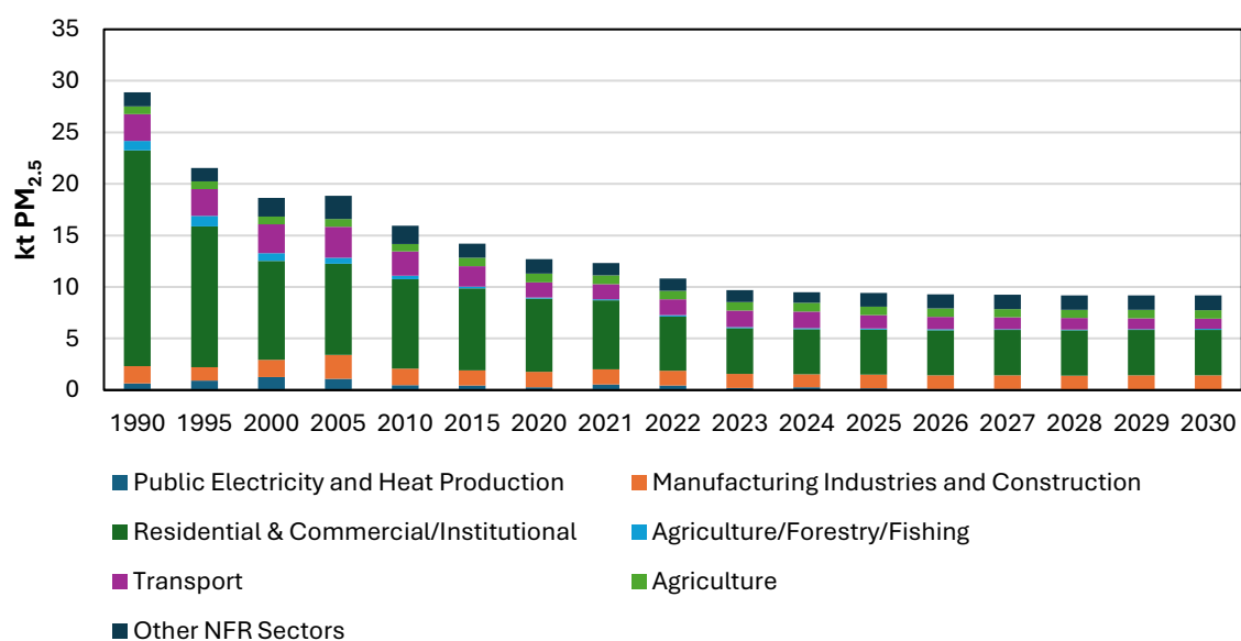
Figure 8.13 PM 2.5 Emission Projections for the With Additional Measures Scenario by Source Sector
