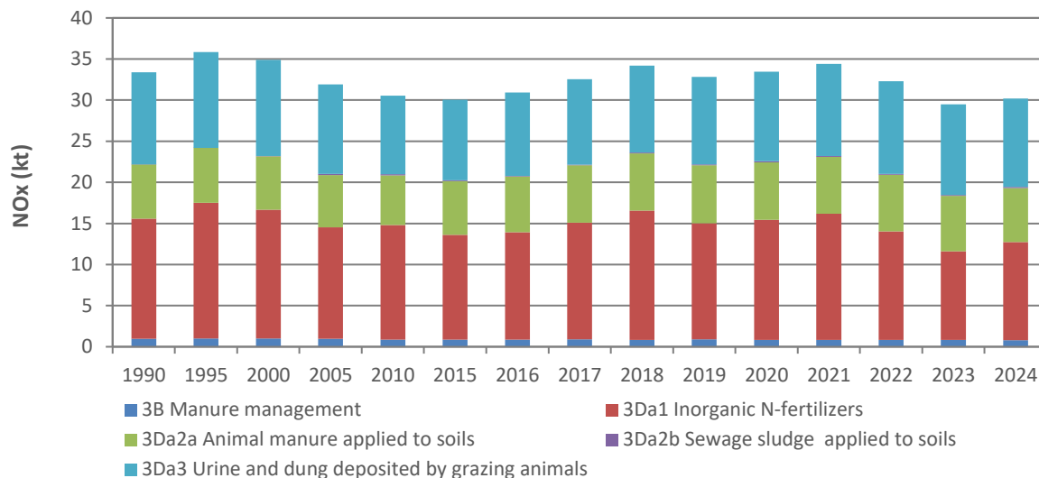
Figure 5.3. Emissions Trend for NO x from Agriculture 1990–2024
