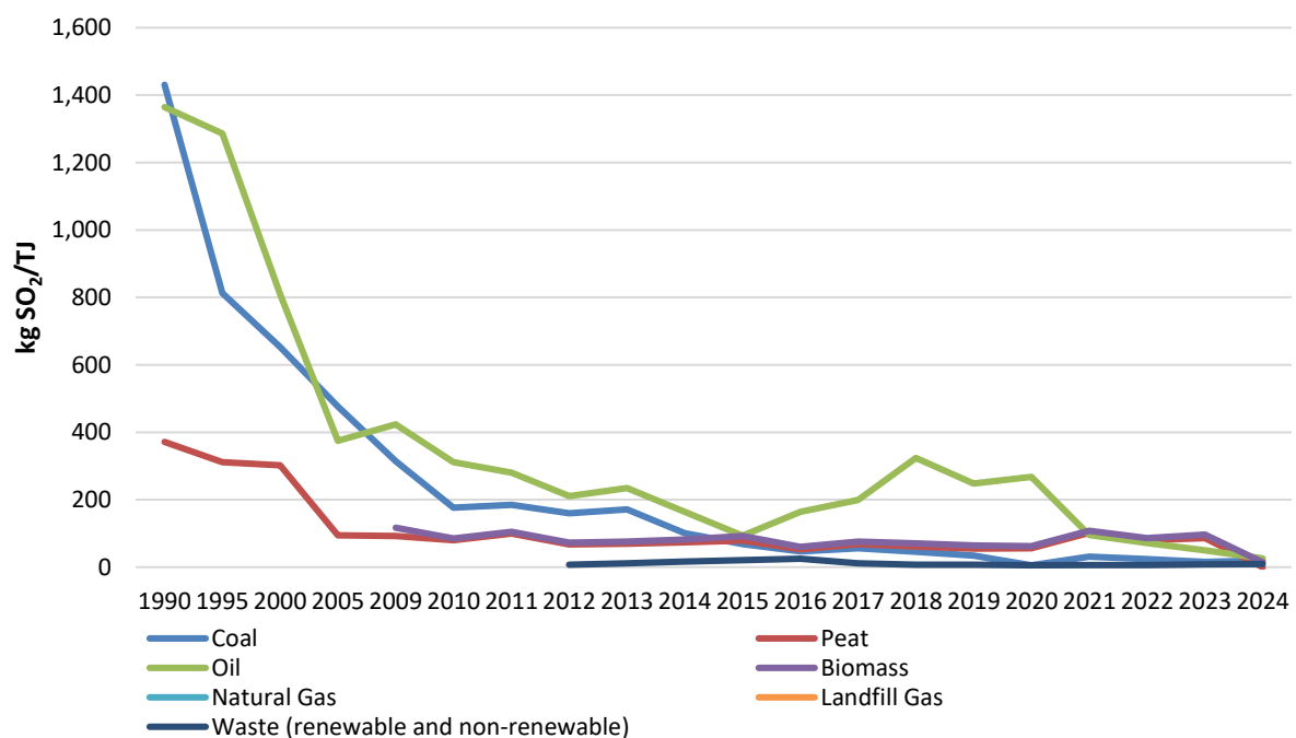
Figure 3.2 Sulphur Dioxide Implied Emission Factors (IEF) for Category 1A1a
