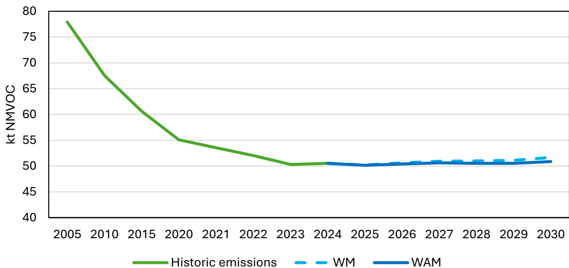
Figure 8.11 NMVOC Emission Projections for the With Existing Measures and With Additional Measures Scenarios where an adjustment is applied for category 3B1a, 3B1b and 2H2 Spirit production under Gothenburg Protocol
