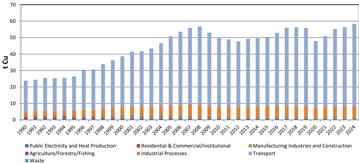
Figure 2.15 Emission Trend for Copper 1990–2024
