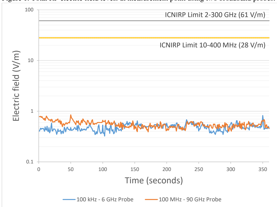
Figure 1. Total RF electric field levels at measurement point using two broadband probes.
