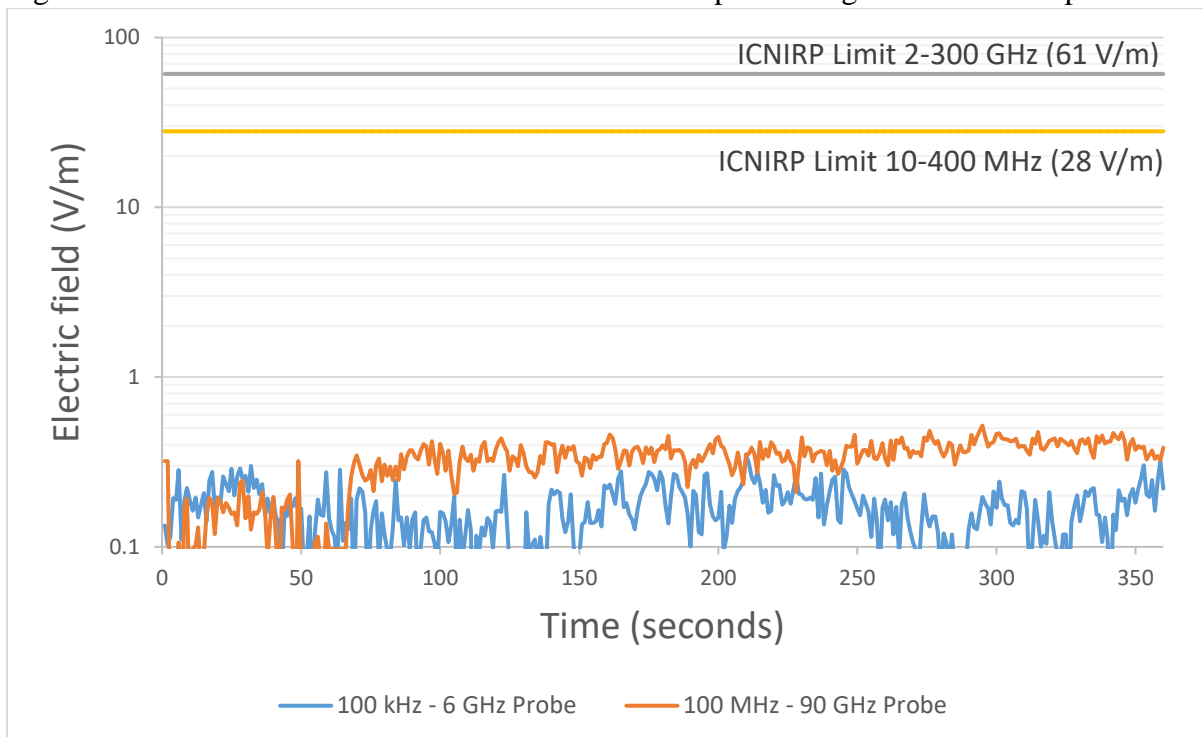
Figure 1. Total RF electric field levels at measurement point using two broadband probes.
