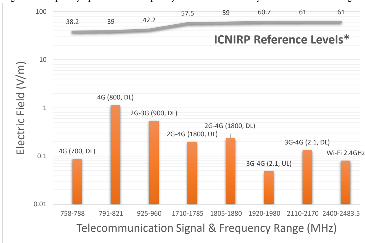
Figure 2. Frequency-specific radiofrequency electric field level by telecommunication signal
