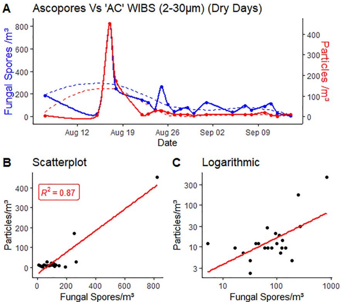
Figure 3.8. (A) Time series of Hirst ascospores and WBS AC particle concentrations (days with 1 mm of rainfall or less); (B) linear scatterplot of daily values ( R^2=0.87 ); (C) logarithmic scatterplot of daily values.
