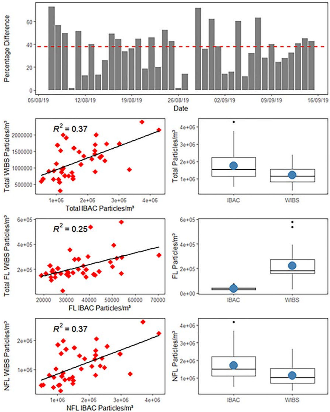
Figure 4.3. Comparison between the WBS-NEO and the IBAC-2 of total, fluorescent and non-fluorescent particle concentrations in the size range 0.7–10 µm.
