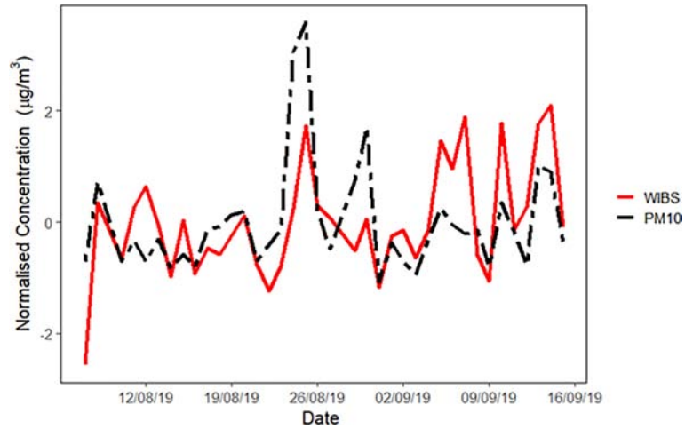
Figure 4.5. Normalised comparison of concentrations of WBS particles and \text{PM}_{10} (dust) emissions during the monitoring campaign.
