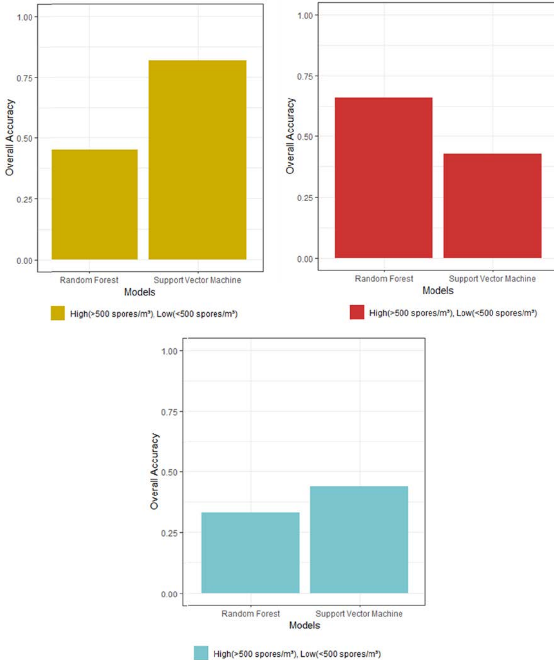
Figure 5.2. Comparison of the accuracy of the results from the Cladosporium classification model using data from three sites.
