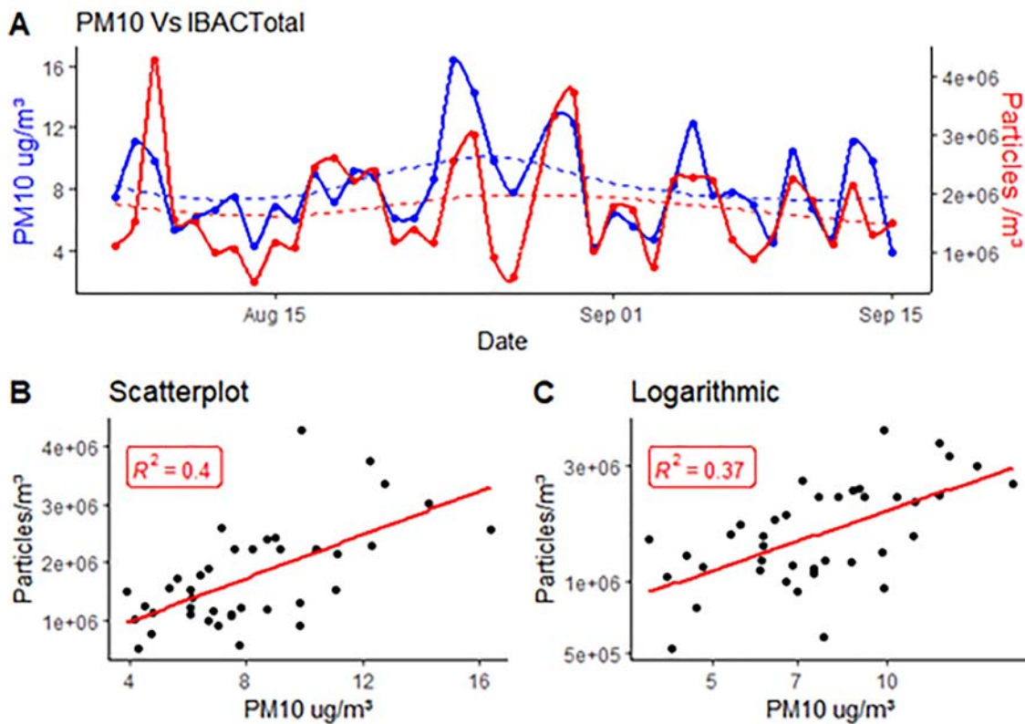
Figure 4.4. Comparison of concentrations of IBAC-2 particles and PM 10 (dust) emissions during the monitoring campaign.
