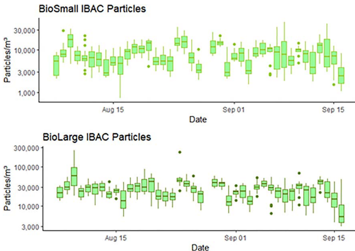
Figure 4.2. Box plots showing daily concentrations of small biological (0.7–1.5 \mu\text{m} ) and large biological (1.5–10 \mu\text{m} ) particles detected by the IBAC-2.
