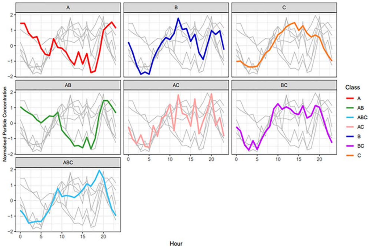
Figure 3.10. WIBS-NEO diurnal charts for each band (particles > 2 μm, 3-sigma).
