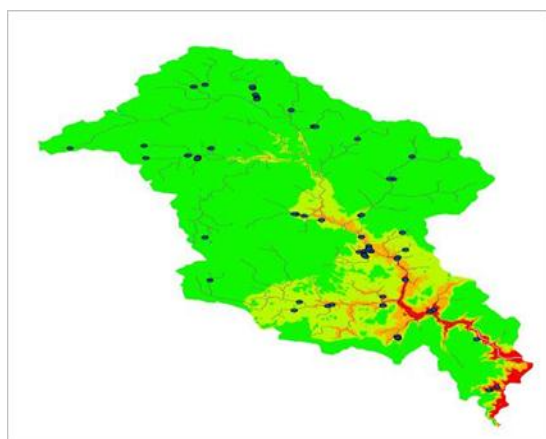
Barrow catchment
