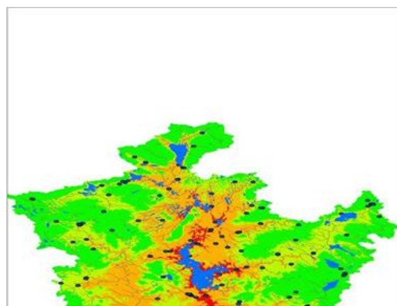
Moy Catchment
