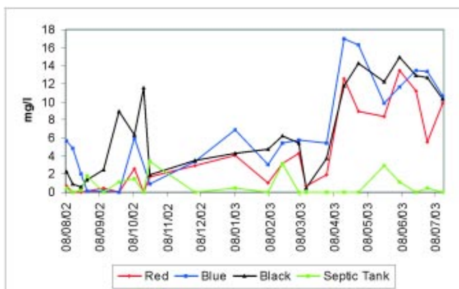
Figure 4.3. NO 3 -N concentrations measured on Site 1.
