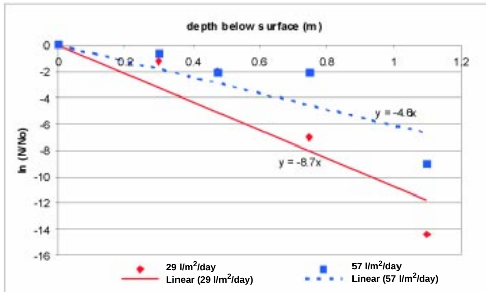
Figure 6.2. Removal of total coliforms with depth through the sand filter (Site 3). N, number of bacteria; N 0 , original number from septic tank.
