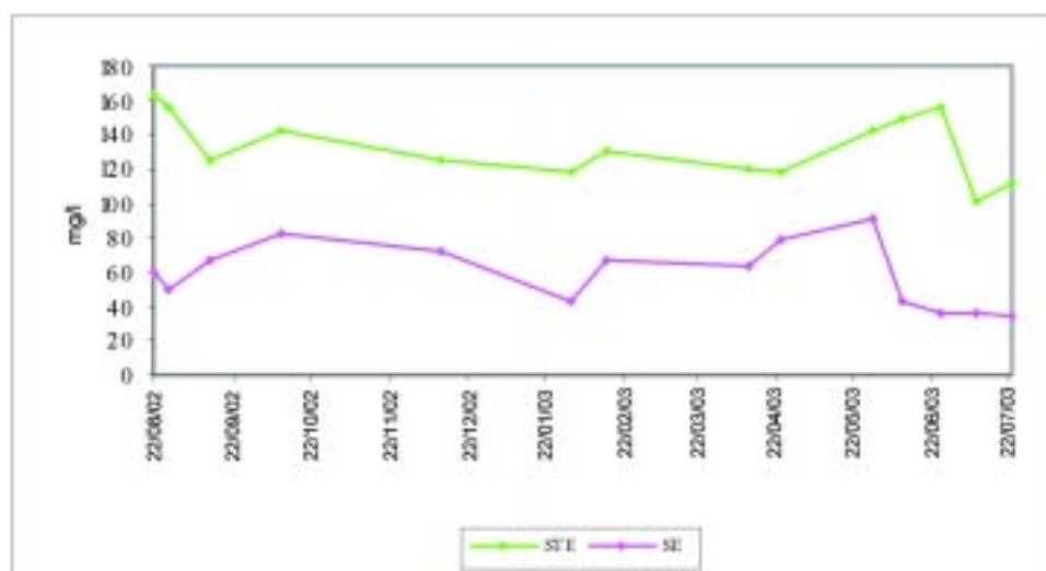
Figure 5.1. Reduction in total inorganic N concentration across the secondary treatment system.
