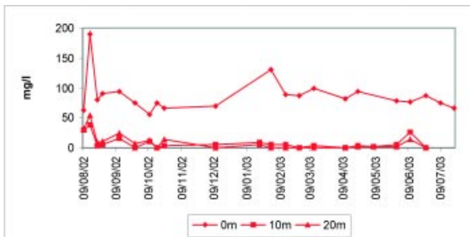
Figure 5.2. Cl concentration on the red depth plane at the three sample positions.
