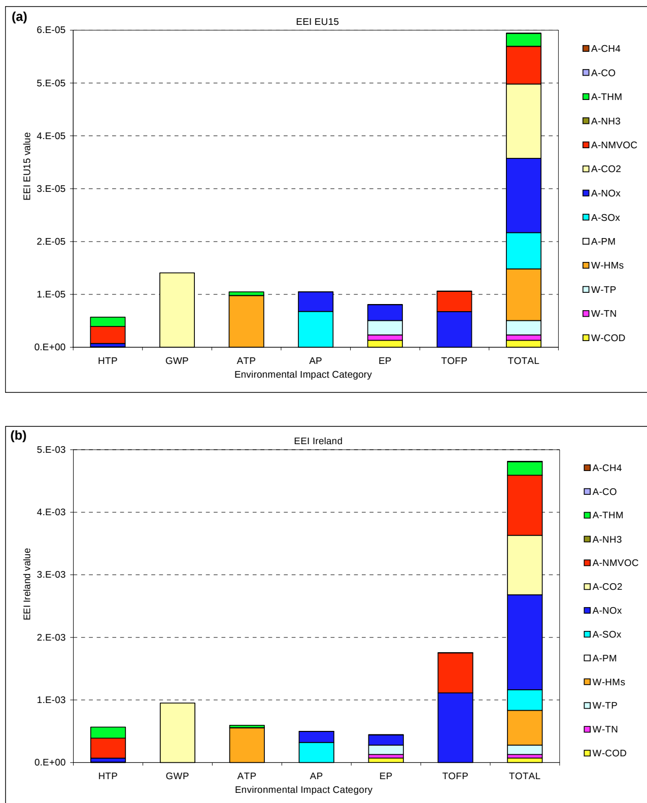
Figure 2.4. The contribution of emissions cumulatively reported by Pharma installations in 2004 towards each impact category, and the final Environmental Emissions Index (EEI) at (a) the EU15 and (b) Ireland scales of context, and (c) in the EU15 European Pollutant Emission Register (EPER) context. HTP, human toxicity potential; GWP, global warming potential; ATP, aquatic toxicity potential; AP, acidification potential; EP, eutrophication potential; TOFP, tropospheric ozone formation potential.
