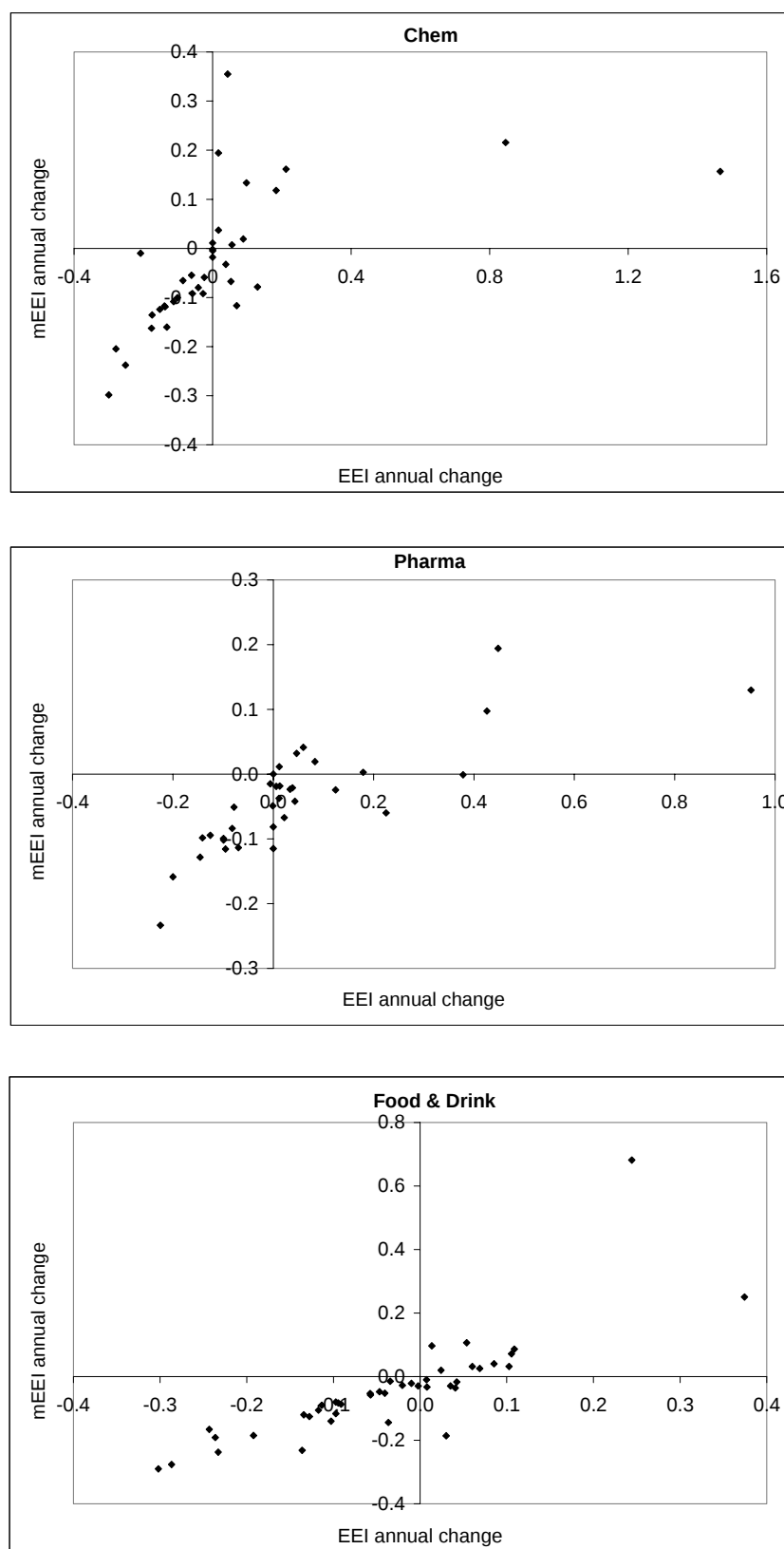
Figure 3.7. Relationships in three sectors between annualised 2004–2007 trends in direct pollution loading (Environmental Emissions Index, EEI) and direct plus indirect electricity generation pollution loading (modified EEI, mEEI) for three sectors. Trends are expressed as average annual fractional change in pollution loading for each installation. Correlation statistics are displayed in Table 3.5 .
