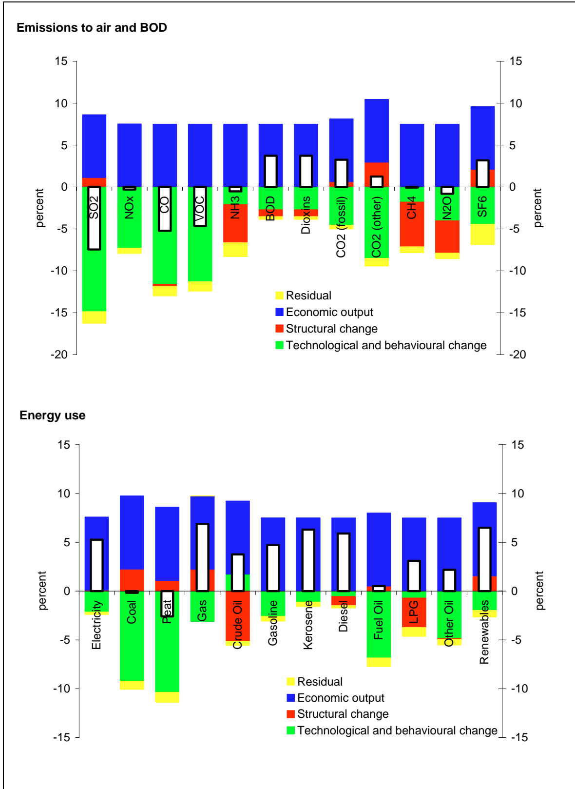
Figure 2.1. A decomposition of the growth rate of emissions and resource use. Note: The average annual growth rate for the period 1990–2006 is presented as the white insert. The growth rate is decomposed into the economic growth rate, the rate of structural change in the economy, technological and behavioural change, and a residual.
